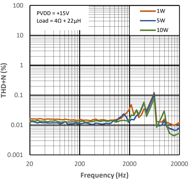
Figure 12-8 THD+N vs Frequency for PMP4
