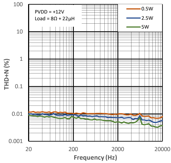
Figure 15-6 THD+N vs Frequency for PMP1
