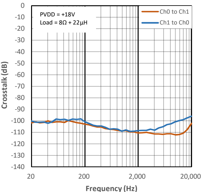
Figure 11-32 Crosstalk vs Frequency for PMP4
