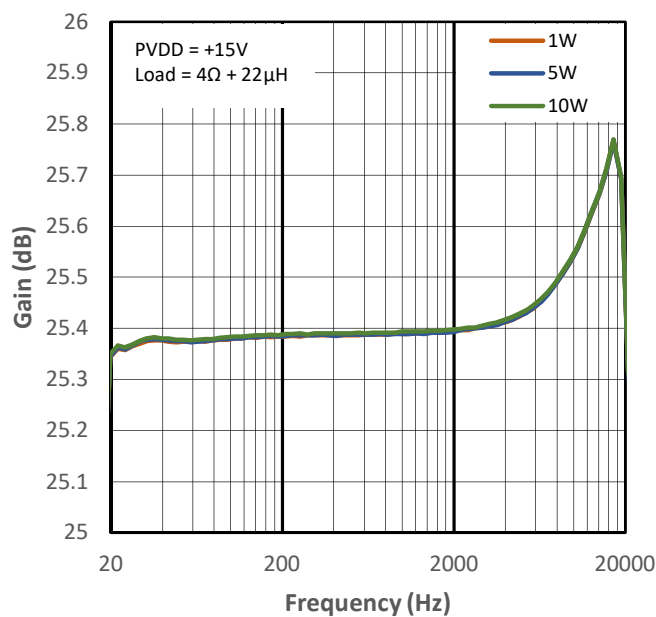
Figure 12-23 Gain vs Frequency for PMP2
