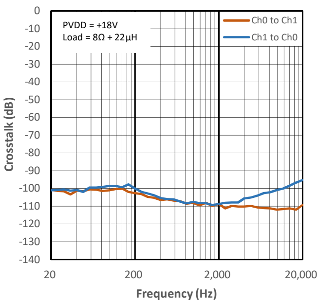
Figure 11-30 Crosstalk vs Frequency for PMP1
