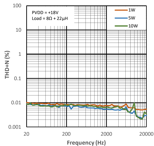
Figure 11-6 THD+N vs Frequency for PMP1
