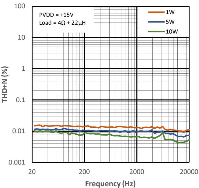
Figure 12-6 THD+N vs Frequency for PMP1
