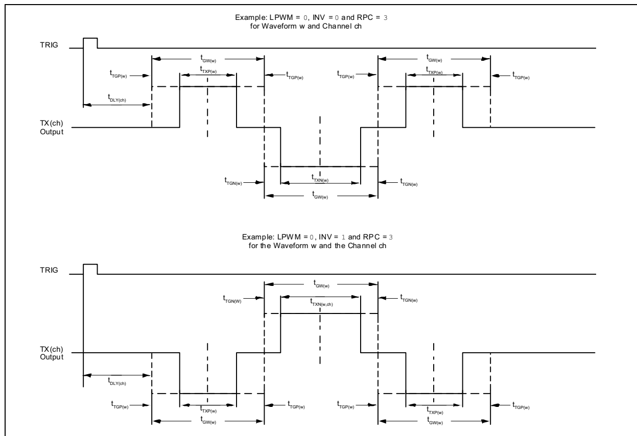
FIGURE 4-12: TX_{CH} Pulses PWM Time-Off Diagram (LPWM = 0).
