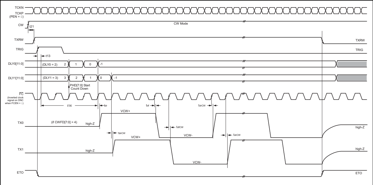
FIGURE 4-6: CW Output Timing Diagram.
