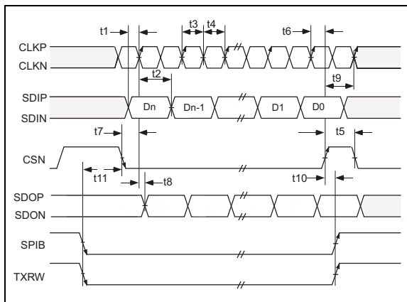
FIGURE 4-4: SPI Register Write Timing with SPIB = 0 , TXRW = 0 .
