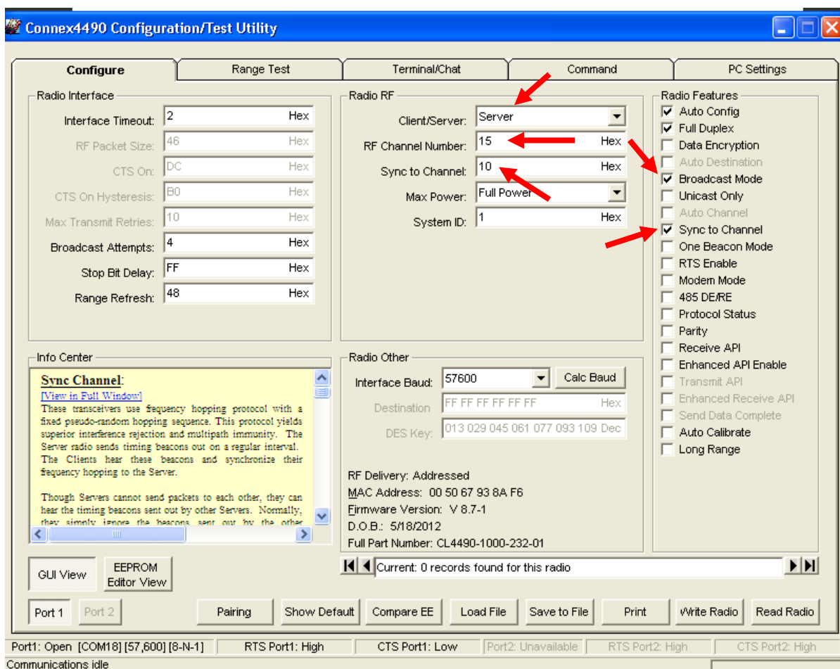
Figure 12: Server #2 settings
