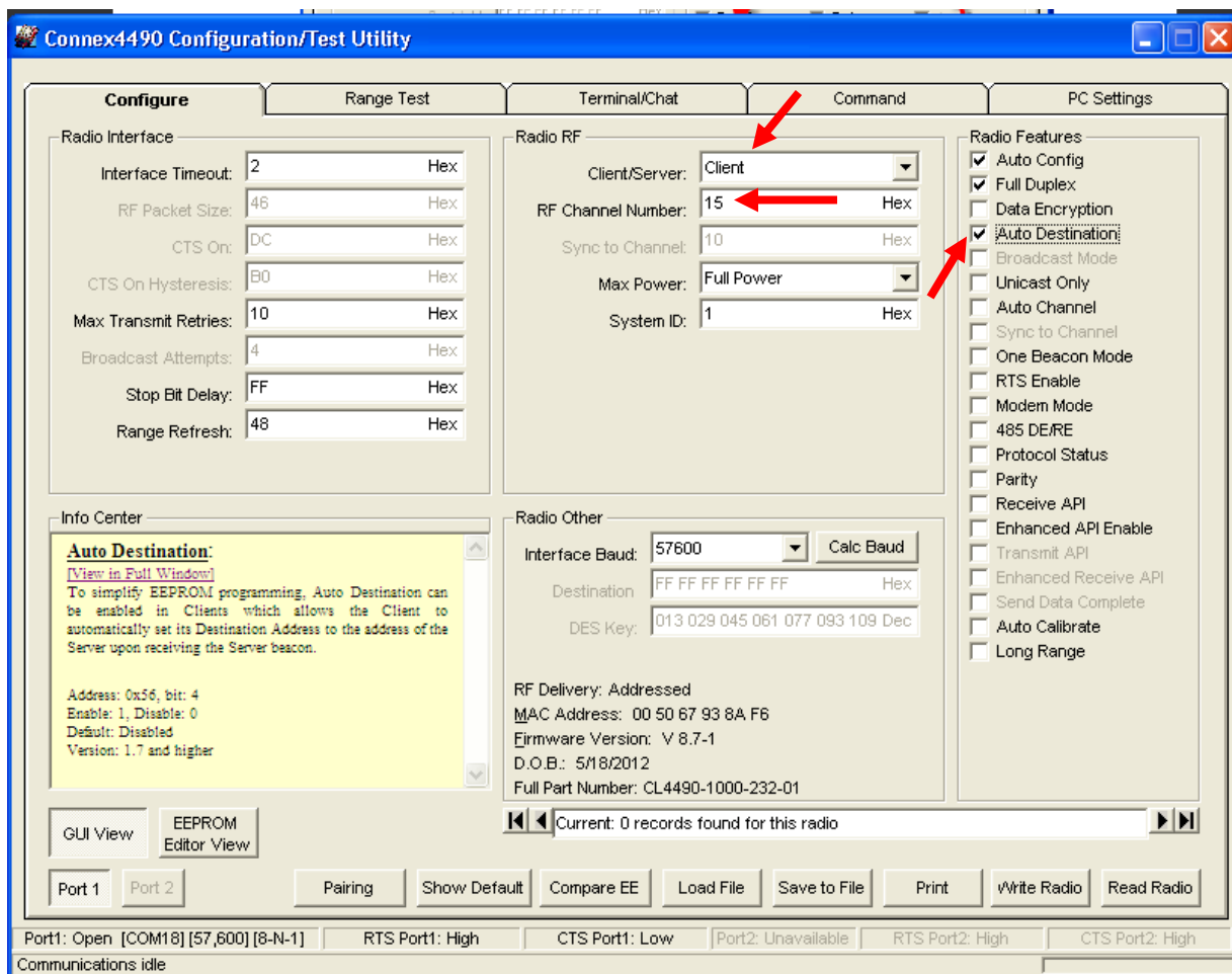
Figure 13: Client settings
