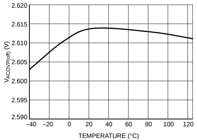
Figure 30. V_{ACOVP(off)} vs. Temperature
