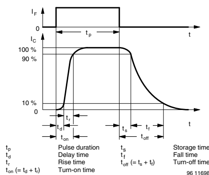
Fig. 2 - Switching Times
