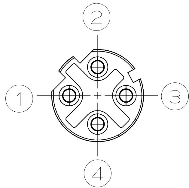
Pin Assignment
