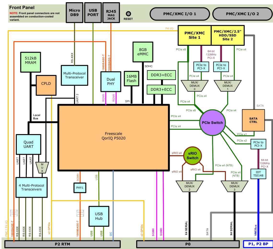
MVME8100 Block Diagram
