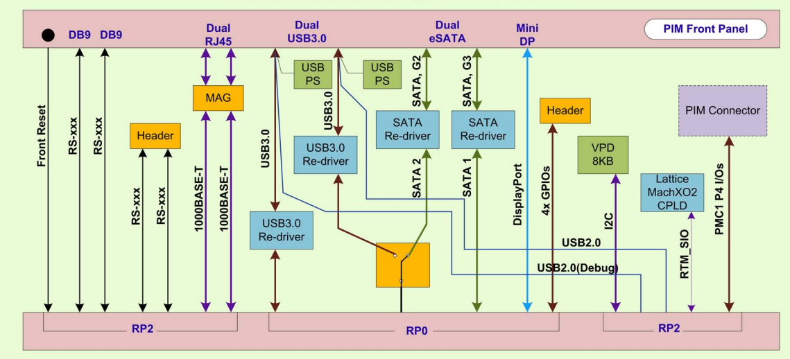
iVME7300/MVME8100 RTM
