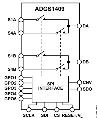
Figure 2. ADGS1409 Functional Block Diagram
