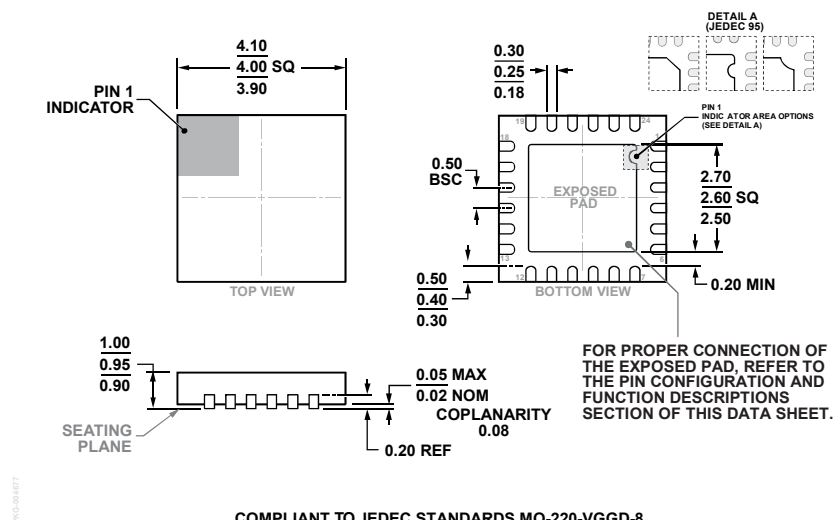
Figure 55. 24-Lead Lead Frame Chip Scale Package [LFCSP]
