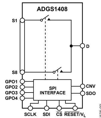
Figure 1. ADGS1408 Functional Block Diagram
