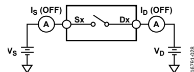
Figure 35. Off Leakage
