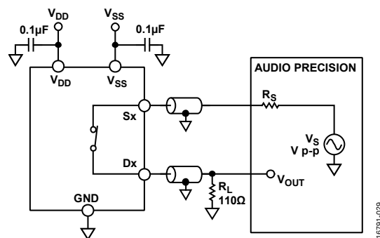
Figure 36. THD + Noise
