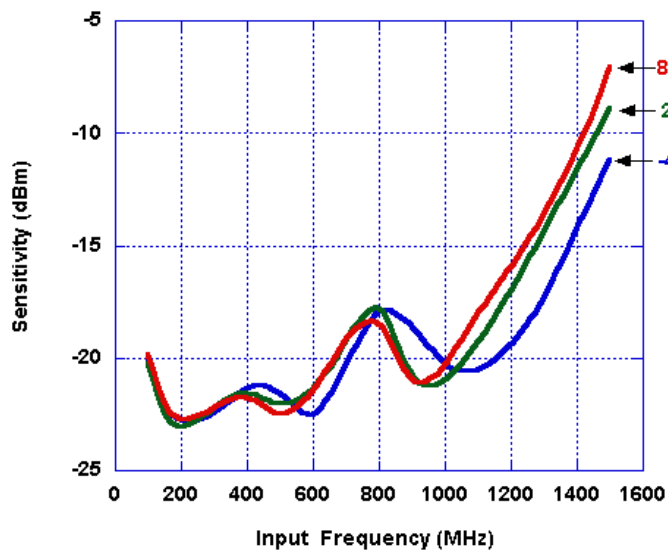
Figure 6. Input Sensitivity
