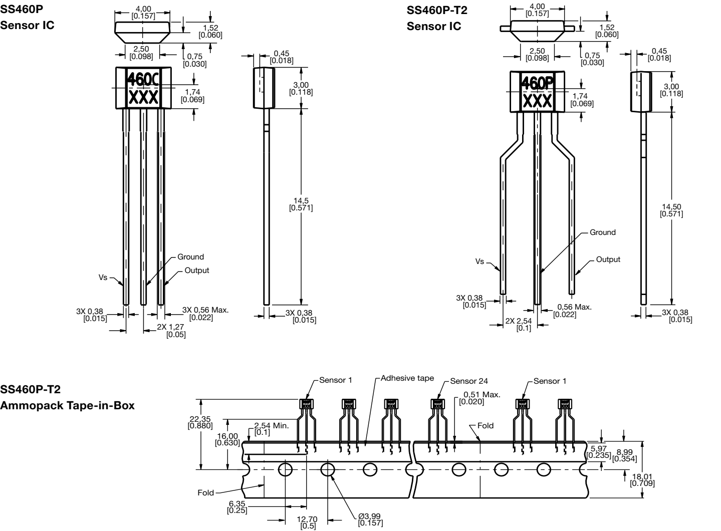
Figure 6. SS460P Sensor IC, SS460P-T2 Sensor IC and Ammopack Tape-in-Box Mounting Dimensions (For reference only. mm/in.)
