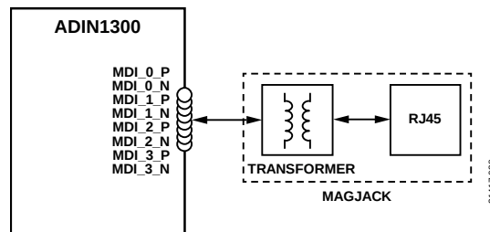
Figure 34. Magnetics Connection
