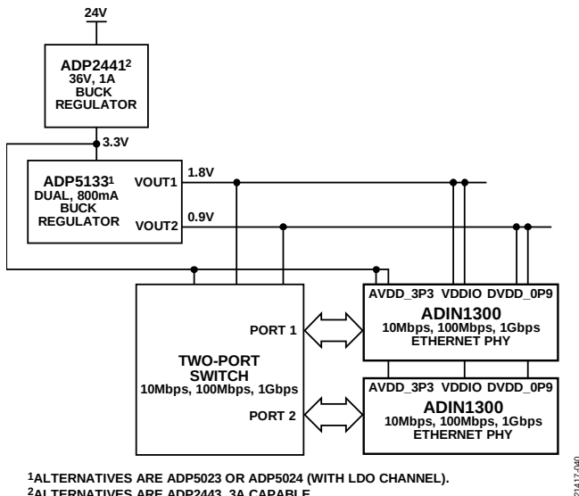
Figure 36. Recommended Power Solution with 24 V System Power, where RGMI is Operating at VDDIO = 1.8 V
