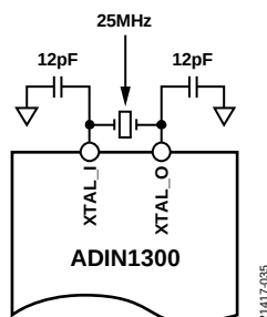
Figure 31. Crystal Oscillator Connection
