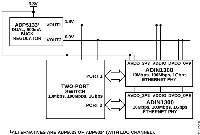
Figure 35. Recommended Power Solution for 3.3 V with RGMI Operating at VDDIO = 1.8 V
