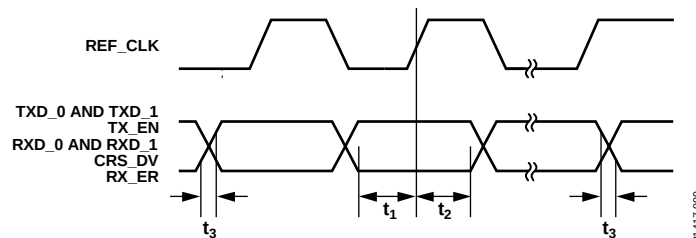
Figure 9. RMII Timing
