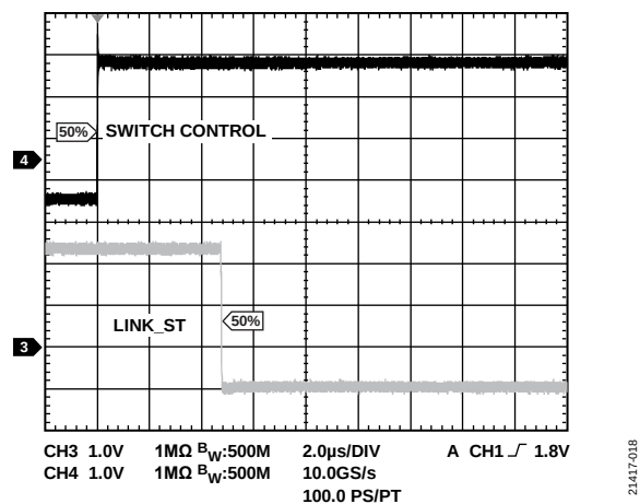
Figure 17. Enhanced Link Detection, 1 Gbps, 100 m Cable with Single Wire Break
