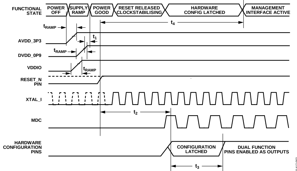
Figure 2. Power-Up Timing
