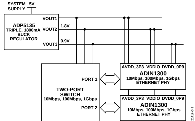
Figure 37. Recommended Power Solution using ADP5135 Triple Buck Regulator to Supply all Three Voltage Rails
