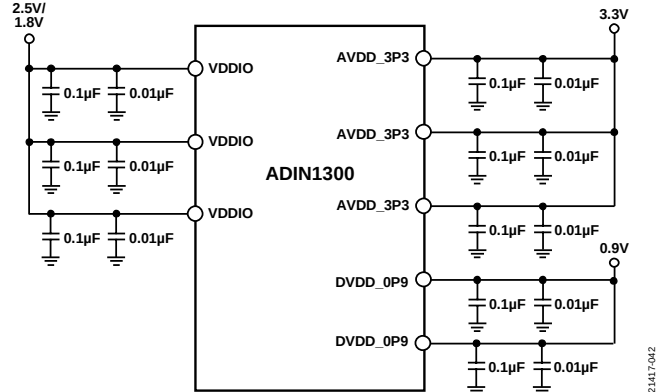
Figure 38. Supply Decoupling Overview
