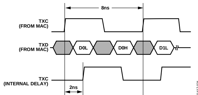
Figure 21. DLL Waveform
