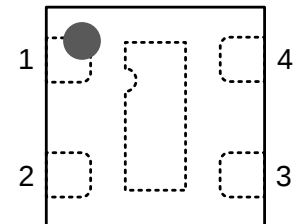
Figure 6. Pin assignment (transparent top view). Dashed lines are only visible if sensor is viewed from below. The die pad is not directly connected to any pin. Pin-1 is indicated by the cutout of the die pad from the bottom side (see dashed lines) and the top side laser marking (dot in upper left corner).
