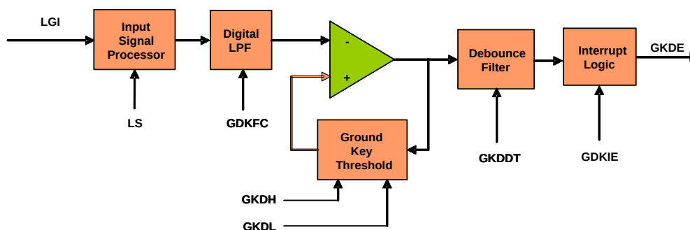
Figure 16: Ground Key Detection Circuitry
