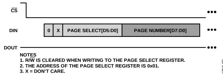
Figure 52. Accessing a Page
