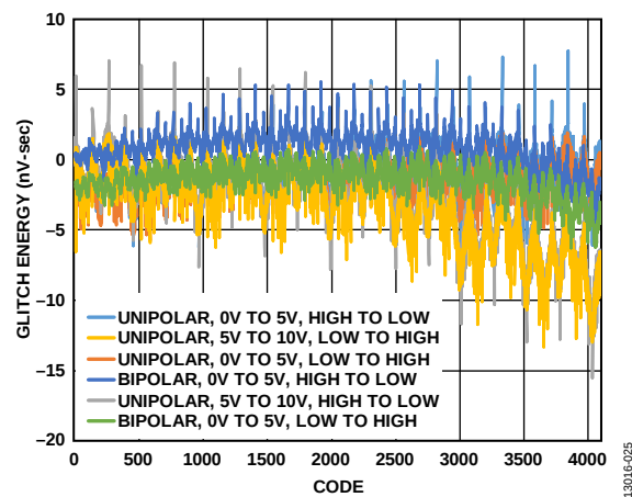
Figure 25. DAC Glitch Energy vs. Code
