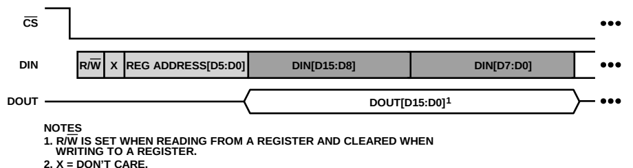
Figure 54. Accessing a 16-Bit Register
