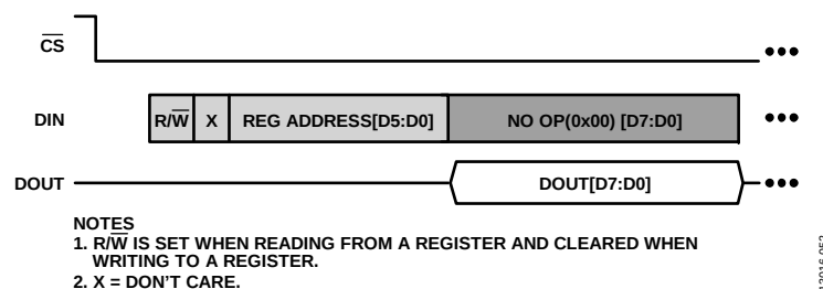
Figure 53. Accessing an 8-Bit Register
