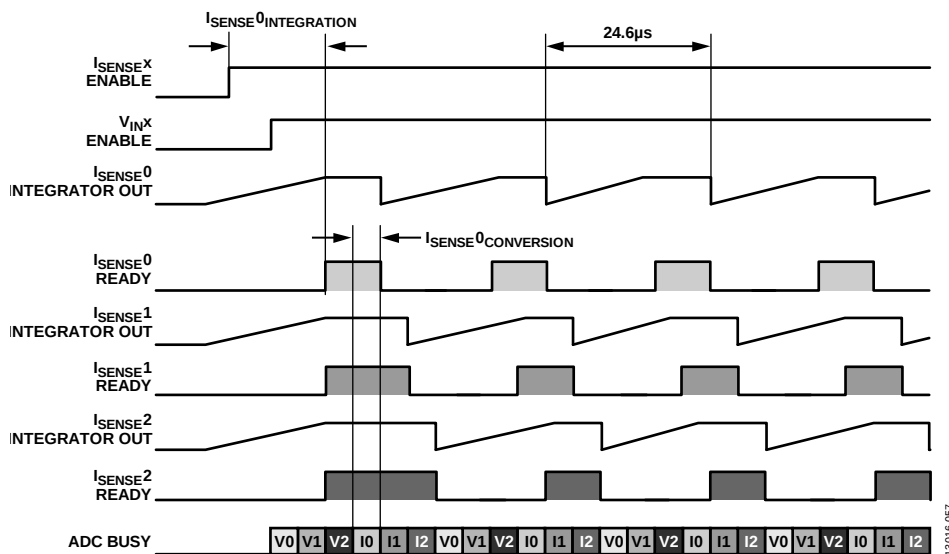
Figure 58. Conversion and Integration Internal Timing Example 2
