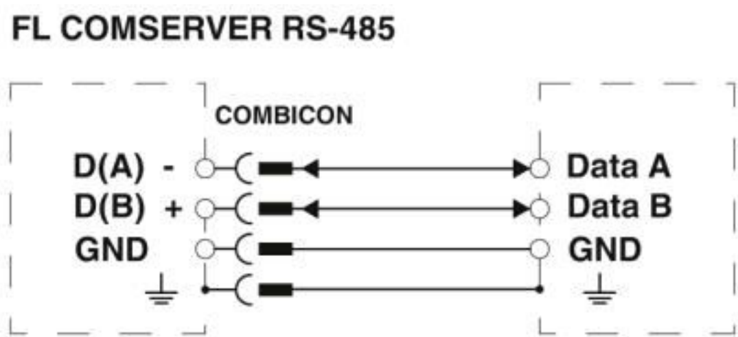
Connection diagram
