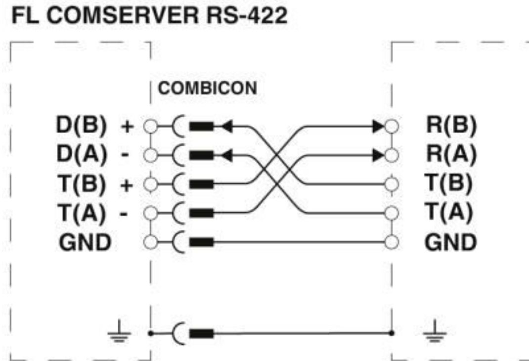
Connection diagram
