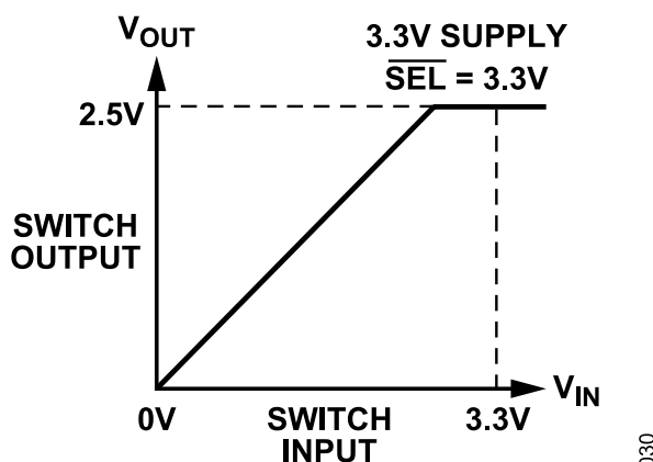
Figure 30. 3.3 V to 2.5 V Voltage Translation, \overline{SEL} = V_{CC}
