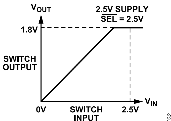
Figure 32. 2.5 V to 1.8 V Voltage Translation, \overline{SEL} = V_{CC}
