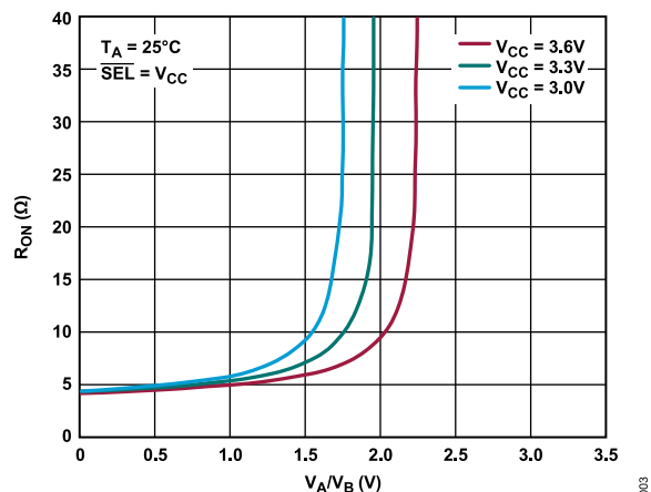
Figure 3. On Resistance vs. Input Voltage, V_{CC} = 3\text{ V} , 3.3\text{ V} , and 3.6\text{ V}
