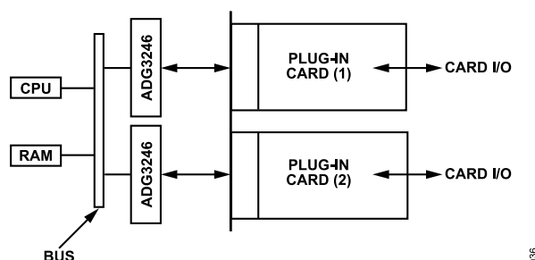
Figure 36. ADG3246 in a Hot Plug Application
