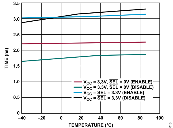
Figure 18. Enable/Disable Time vs. Temperature, V_{CC} = 3.3\text{ V}
