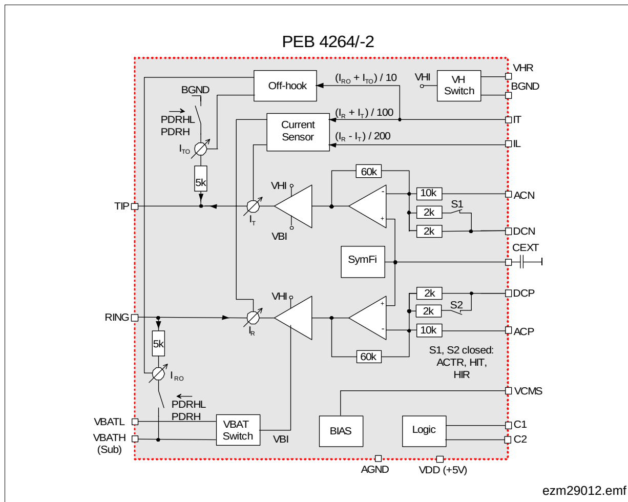
Figure 9 Block Diagram SLIC-S1-S2 (PEB 4264/-2)
