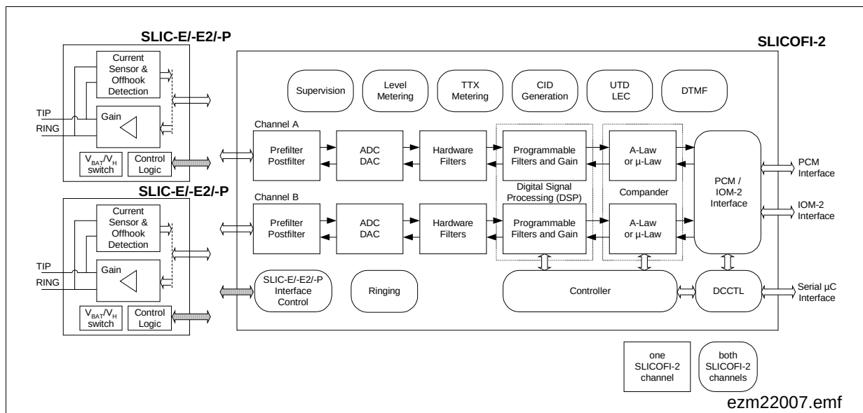
Figure 8 Line Circuit Functions included in the DuSLIC-EI-E2-P
