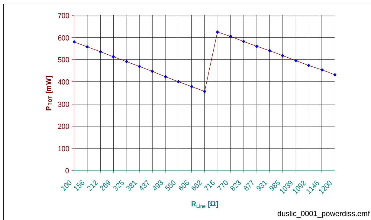
Figure 42 SLIC-P Power Dissipation (Switched Battery Voltage, Long Loops)
