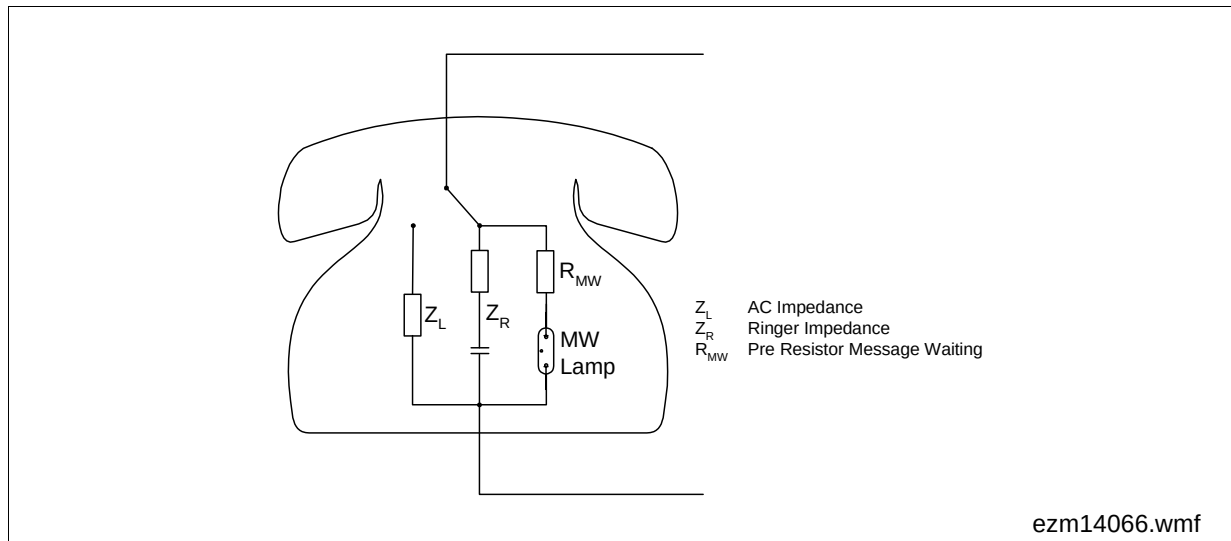
Figure 36 MWI Circuitry with Glow Lamp
