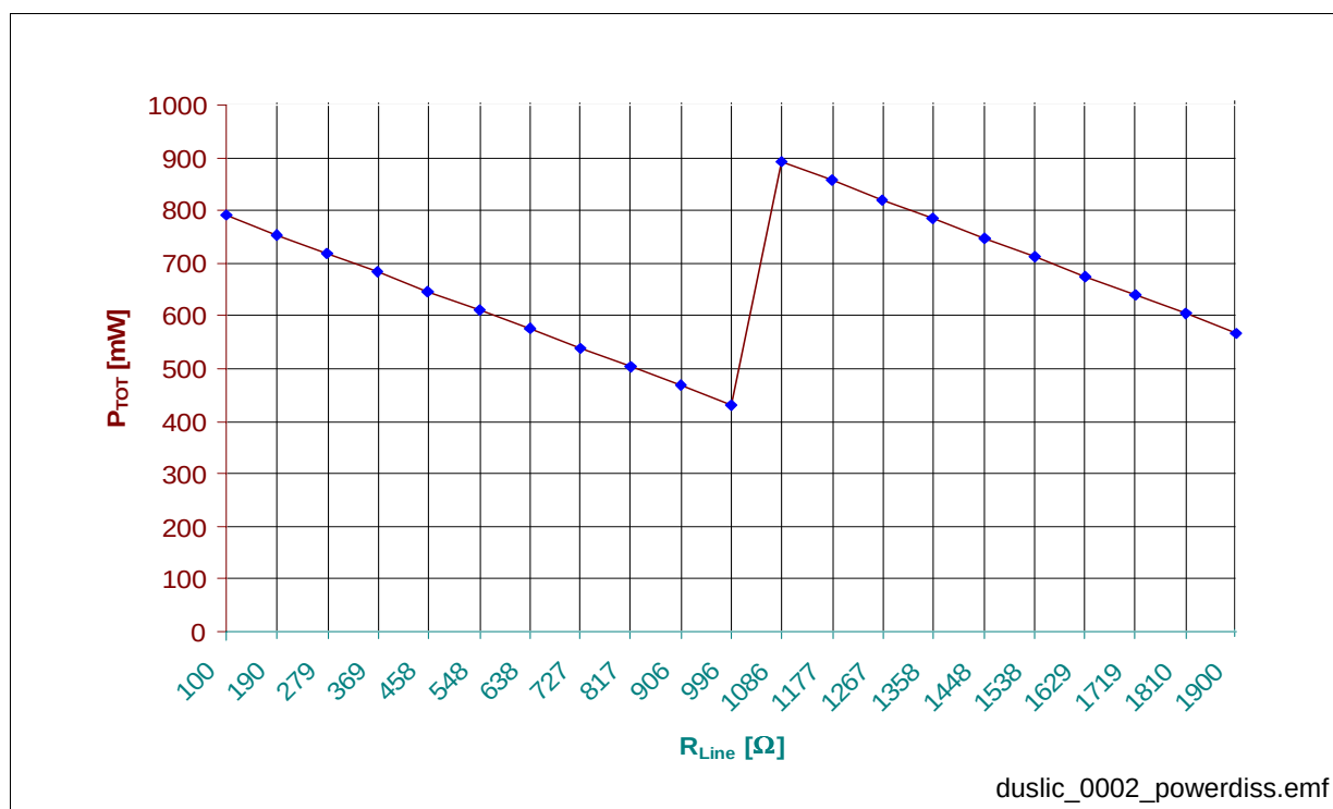
Figure 41 SLIC-E/-E2 Power Dissipation with Switched Battery Voltage
