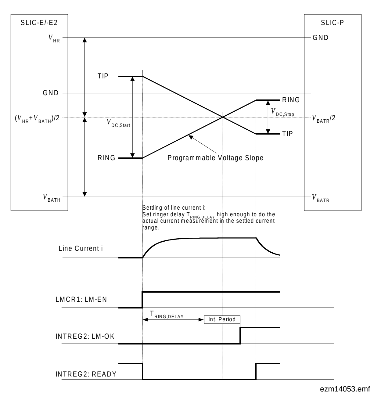
Figure 51 Capacitance Measurement
