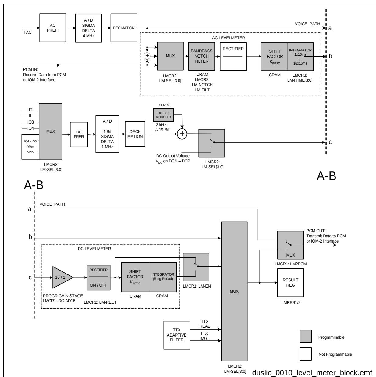
Figure 45 Blockdiagram Levelmeter
