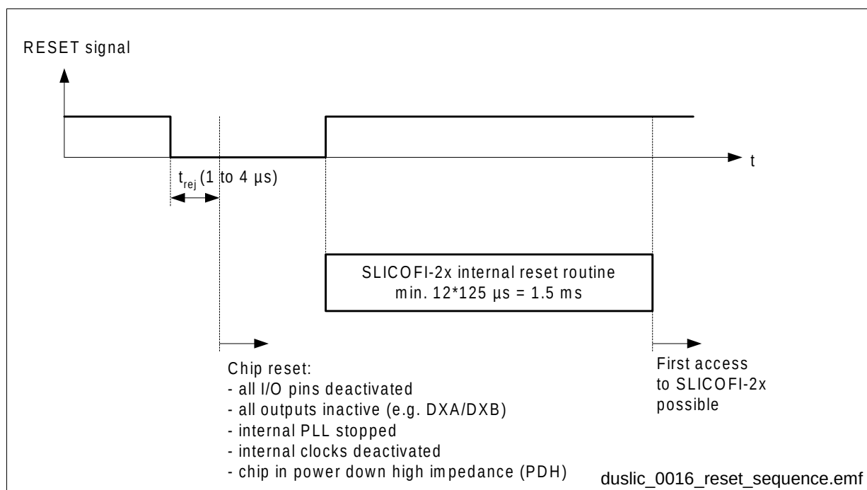
Figure 39 DuSLIC Reset Sequence
