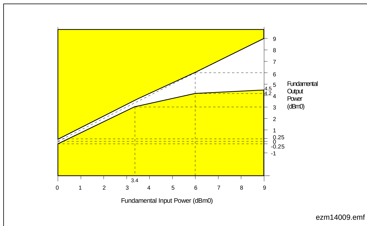
Figure 80 Overload Compression
