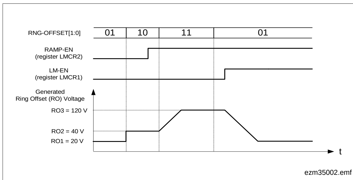
Figure 71 Example for Switching Between Different Ring Offset Voltages
