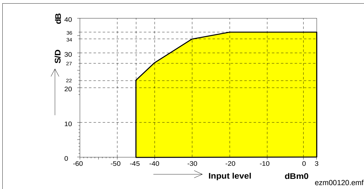
Figure 88 Total Distortion Transmit ( L_x = 0 dBr)
