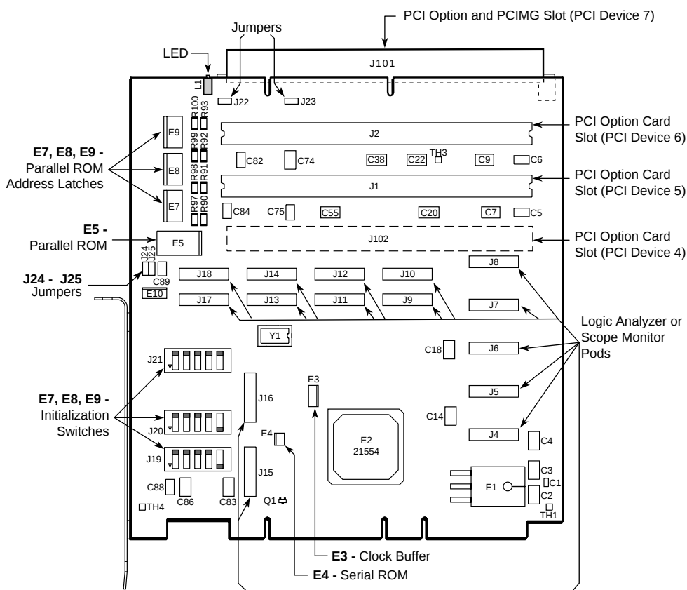
Figure 1-1. Major Components
