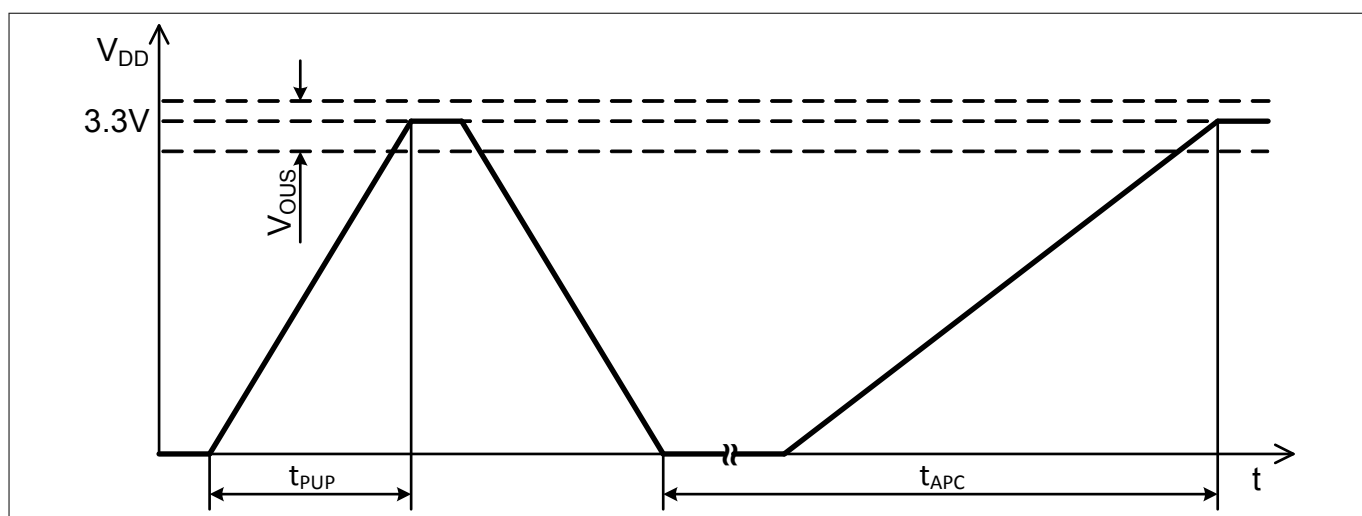
Figure 7 V_{DD} power up and power cycle for high availability
