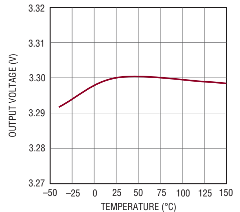
LT3973-3.3 Output Voltage
