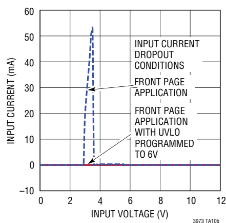
Input Current During Start-Up
