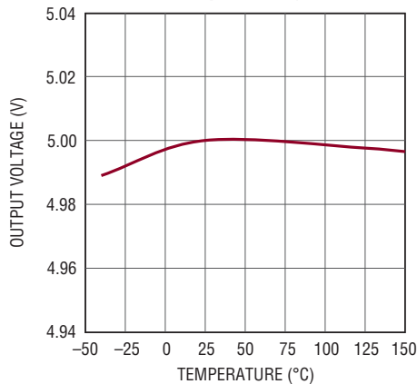
LT3973-5 Output Voltage
