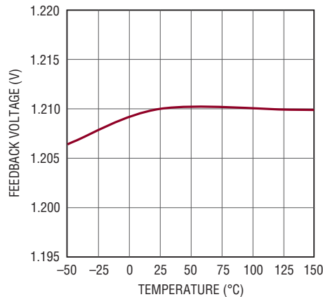
LT3973 Feedback Voltage
