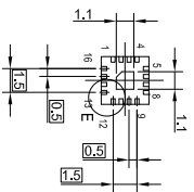
RECOMMENDED IC (REF.)
