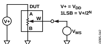
Figure 33. Potentiometer Divider Nonlinearity Error (INL, DNL)
