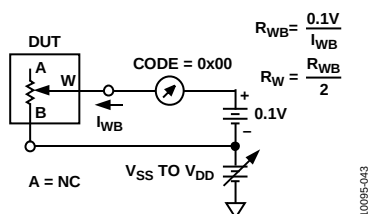
Figure 34. Wiper Resistance
