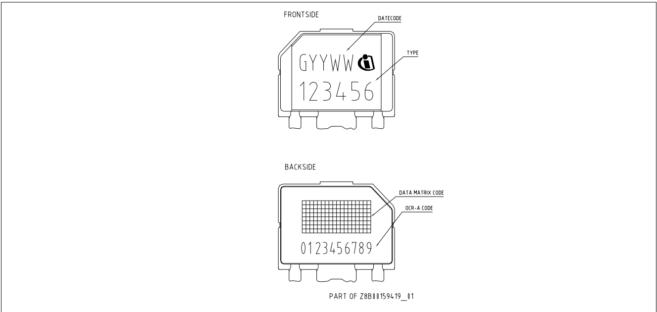
Figure 9 Marking of PG-SSO-3-52 Package
