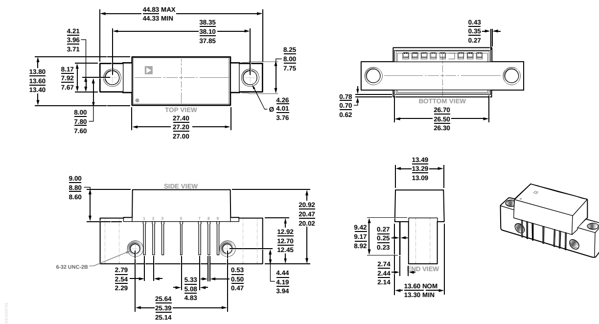
Figure 12. 7-Pin SOT-115J Module Package [MODULE] (ML-7-1)
