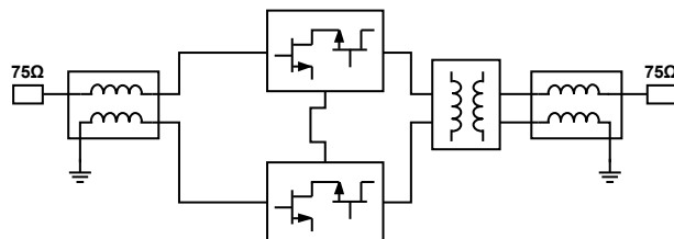
Figure 10. Simplified Schematic
