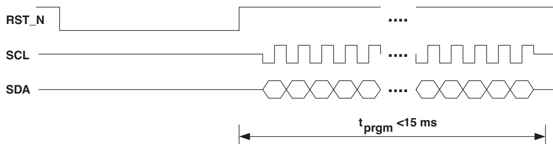
Figure 7. KS8995M EEPROM Configuration Timing Diagram
