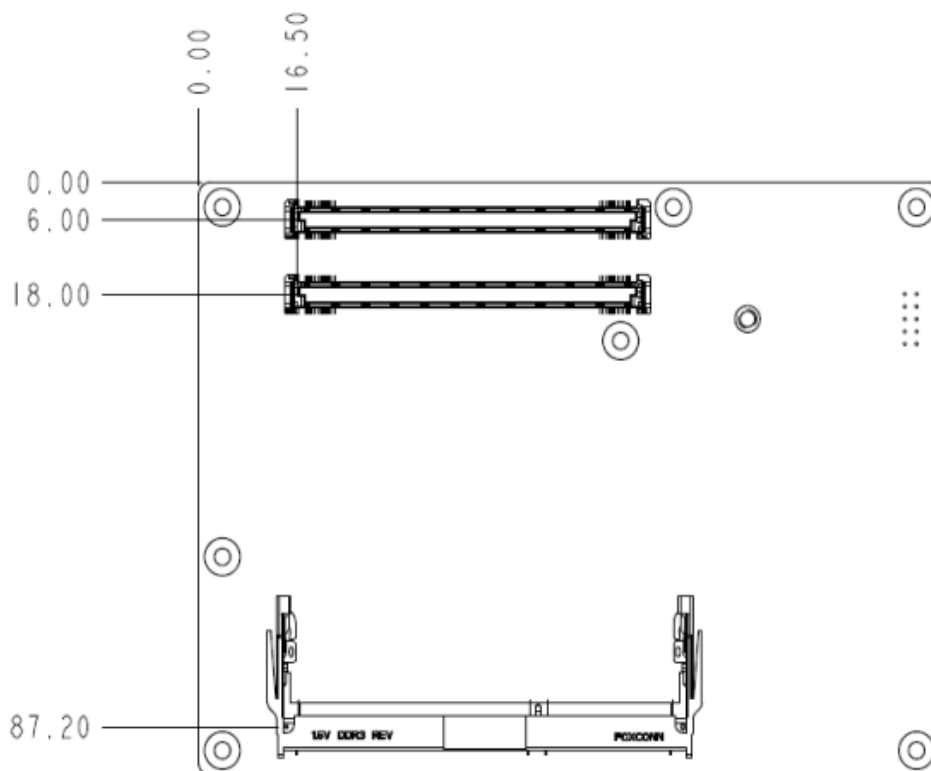
Figure 1-3 COMX-CORE Series Mechanical Dimensions (Rear View)
