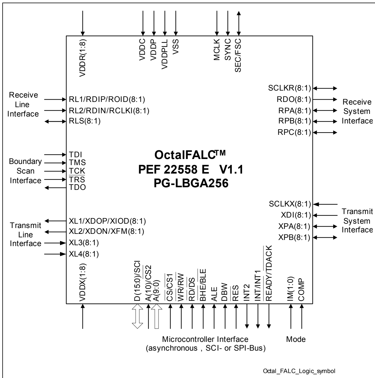
Figure 1 Logic Symbol
