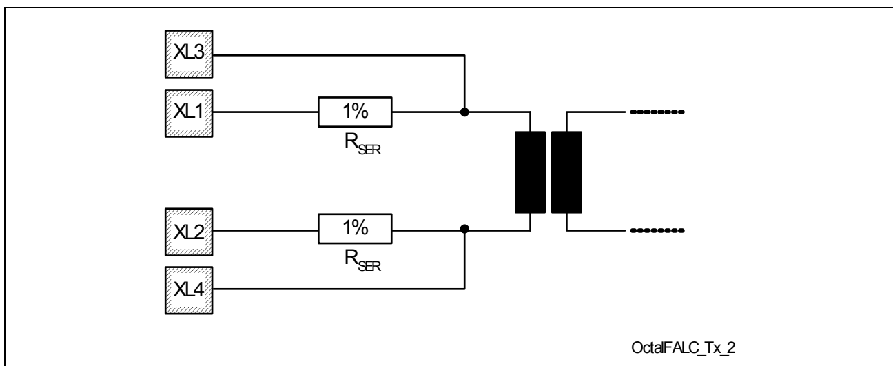
Figure 29 Transmit Impedances
