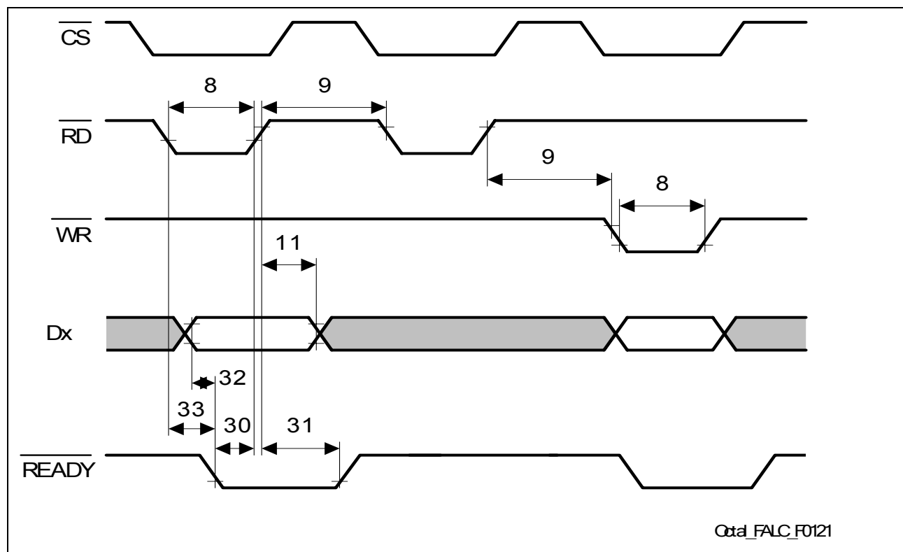
Figure 3 Intel Read Cycle Timing
