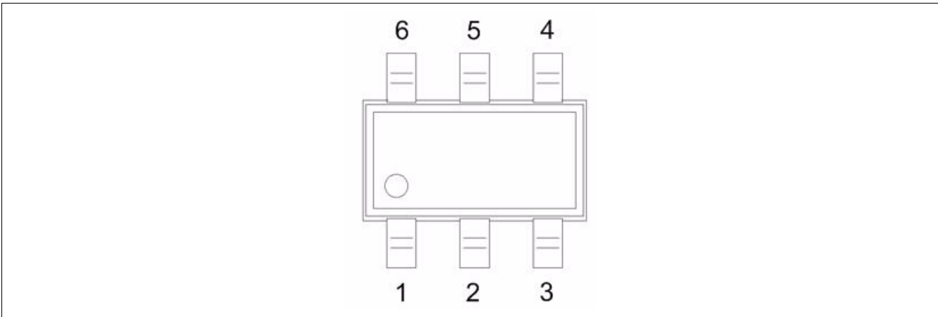
Figure 2 TLI493D-A2B6 pinout
