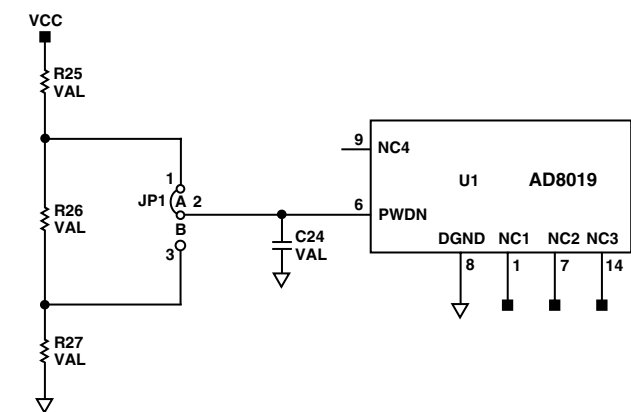
Figure 9. DSL Driver Input Control Circuit
