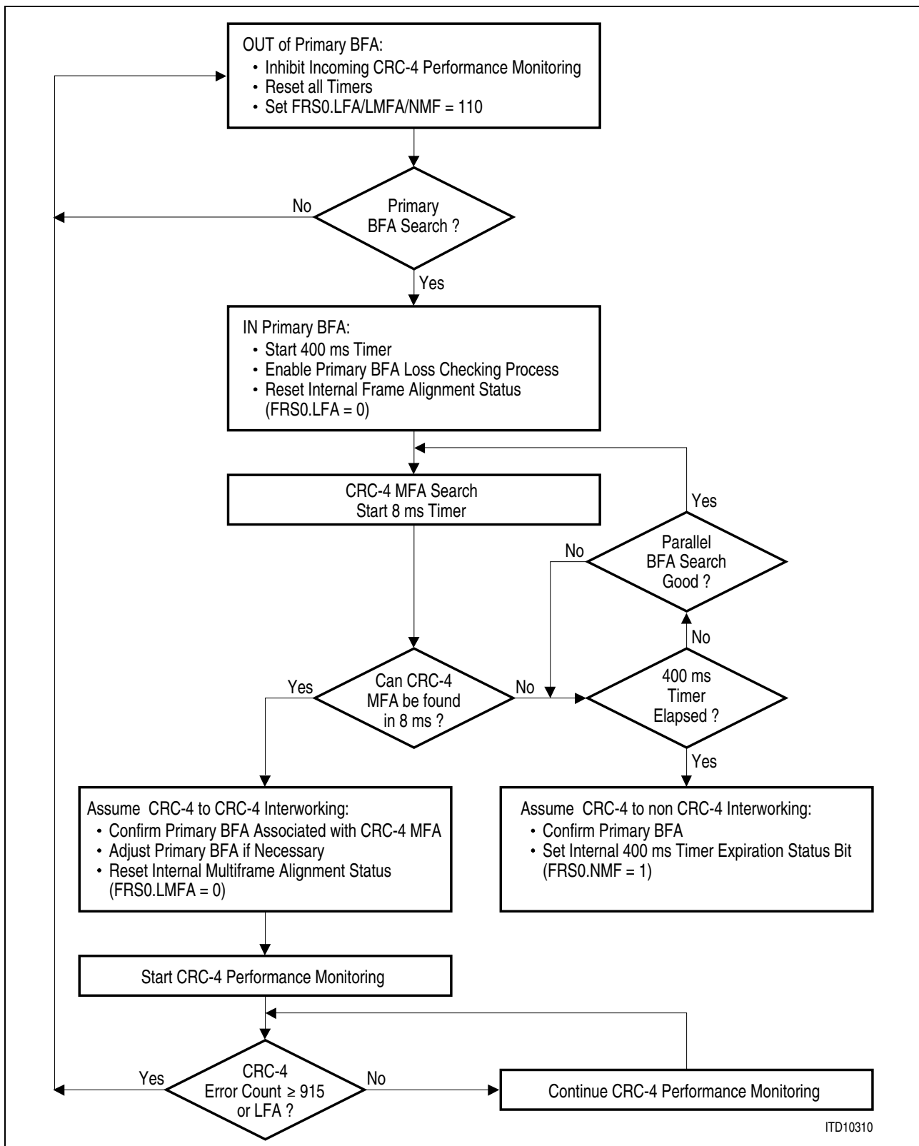
Figure 26 CRC4 Multiframe Alignment Recovery Algorithms (E1)
