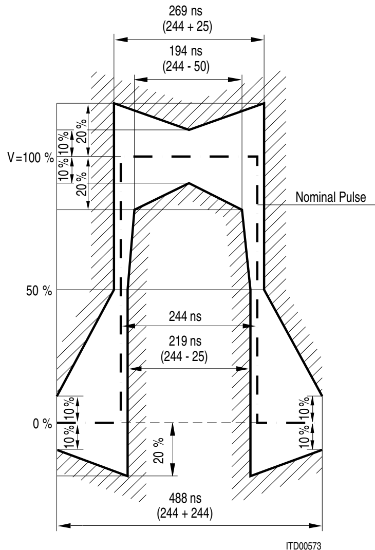
Figure 108 E1 Pulse Shape at Transmitter Output
