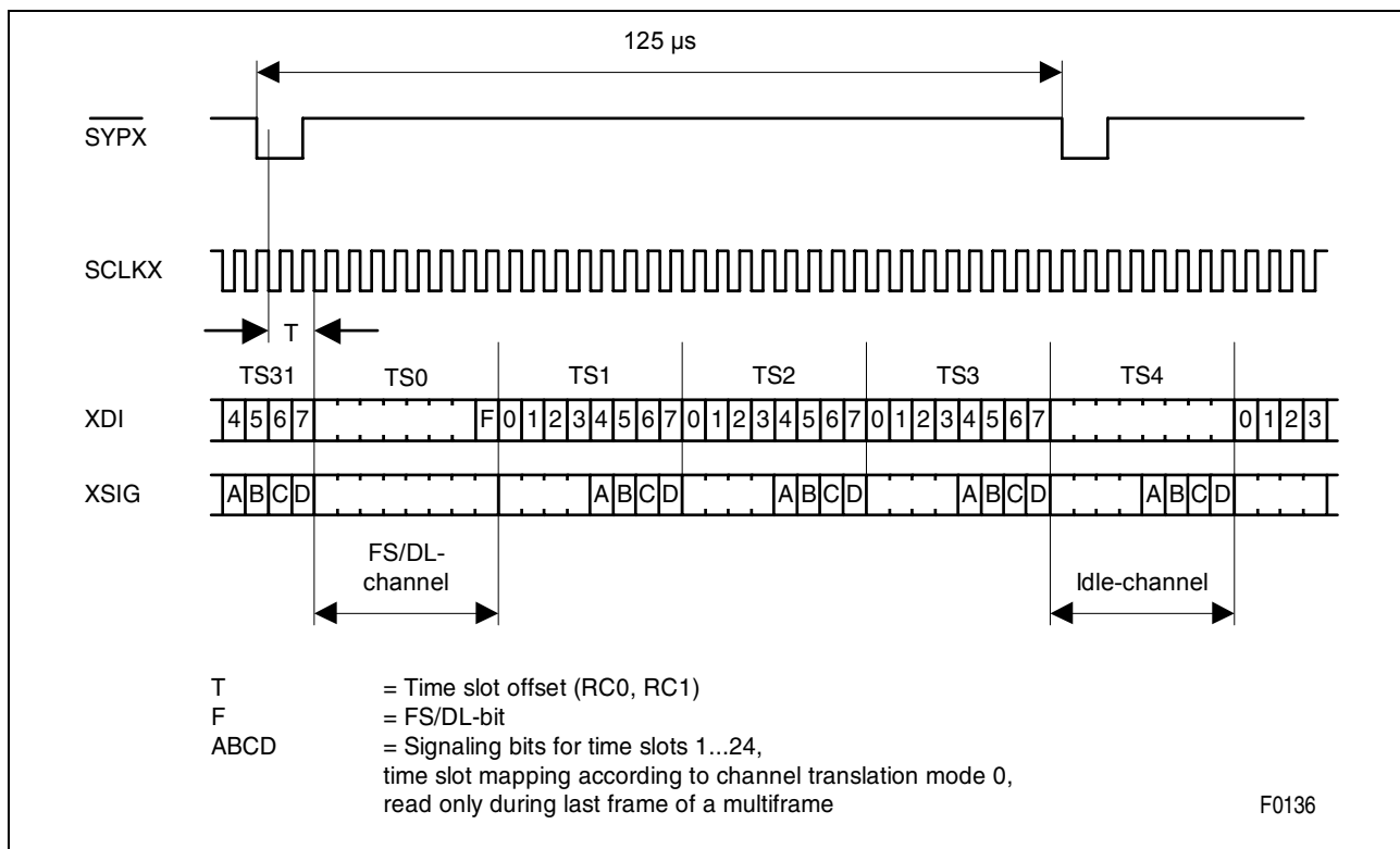
Figure 70 2.048 MHz Transmit Signaling Clocking (T1/J1)
