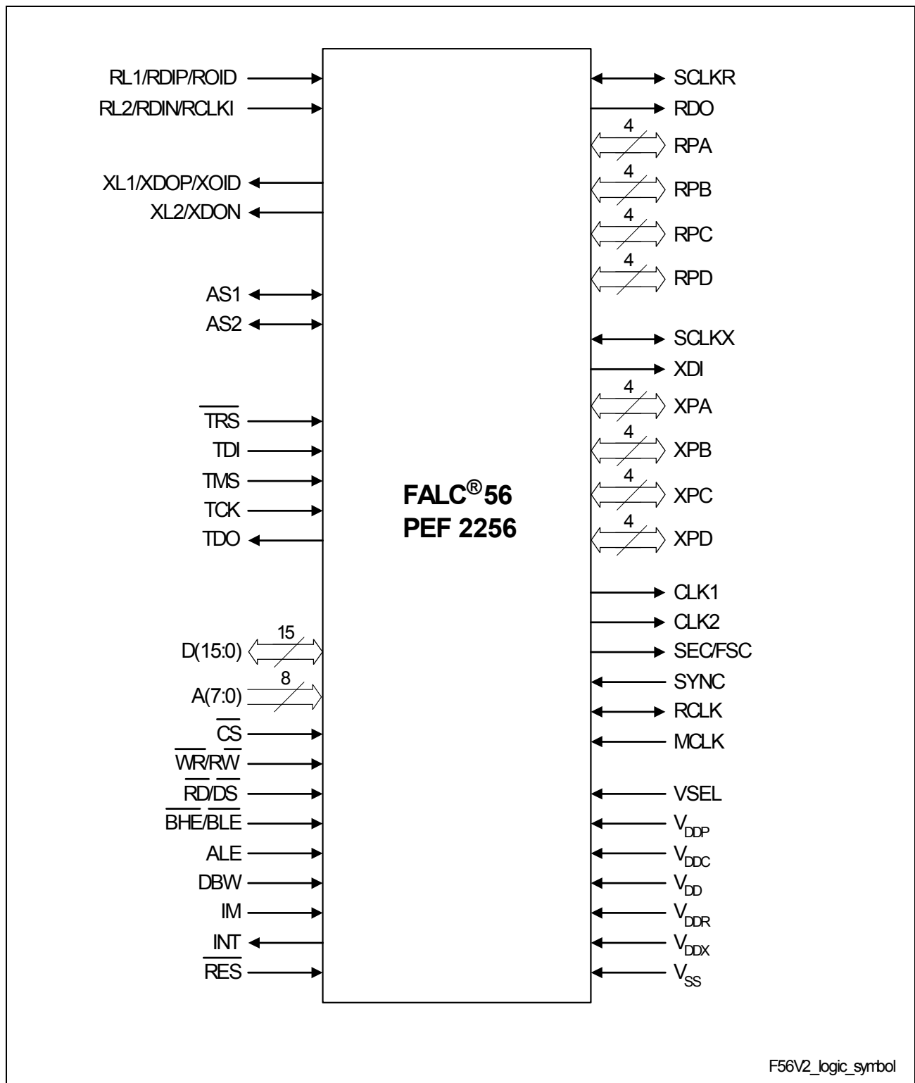
Figure 3 Logic Symbol
