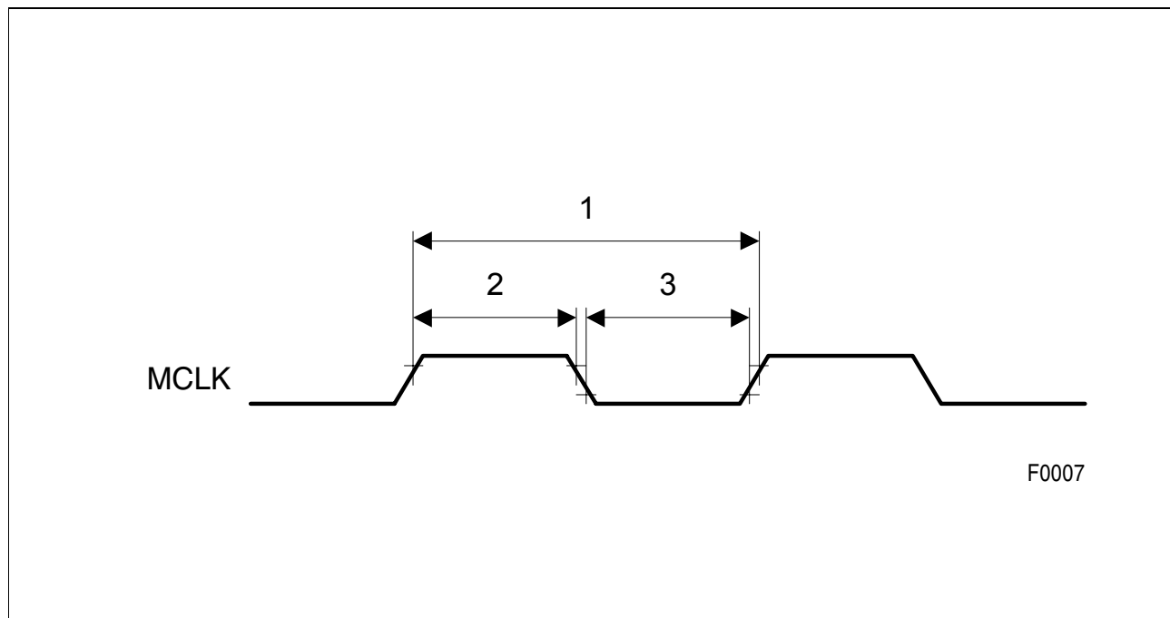
Figure 86 MCLK Timing
