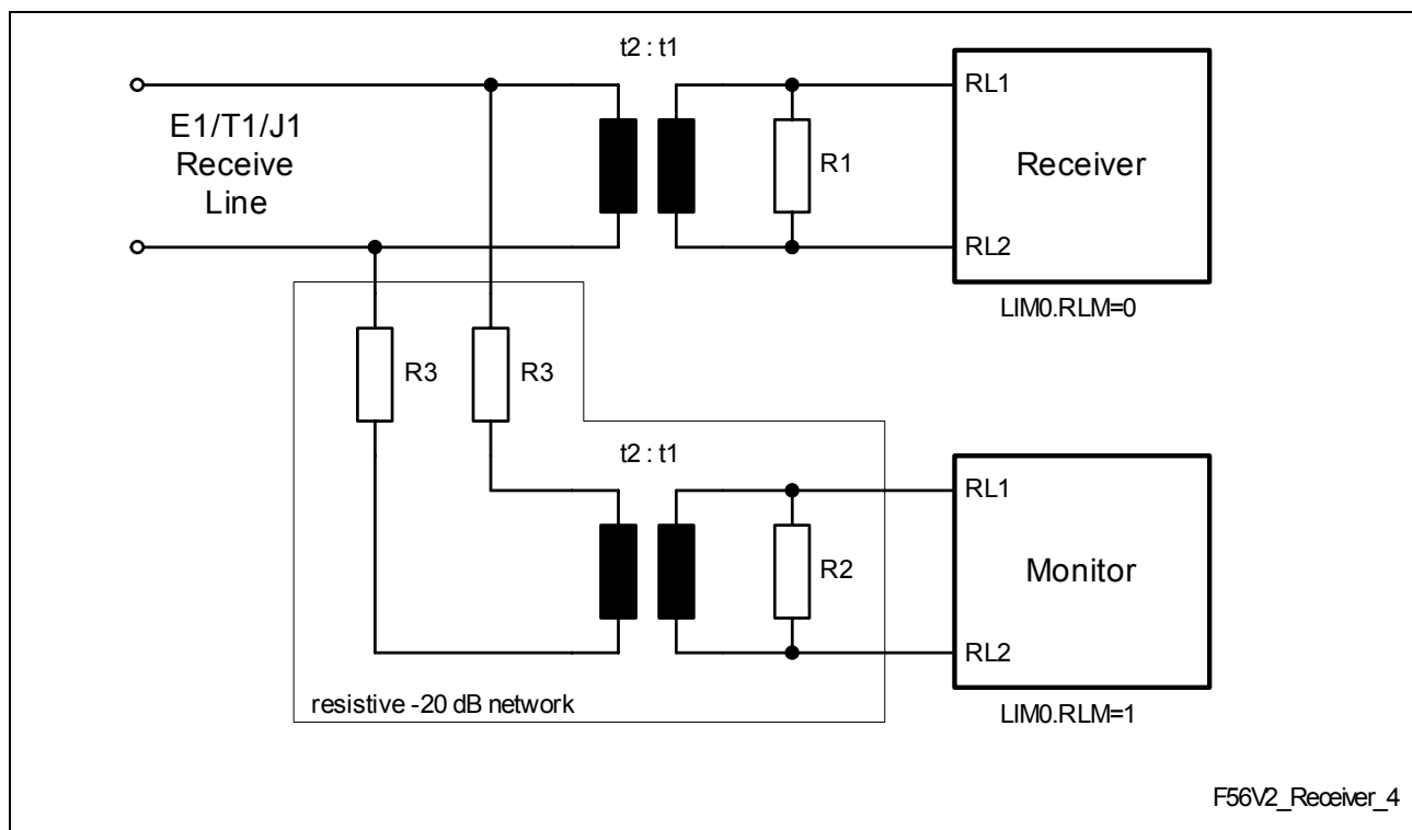
Figure 47 Receive Line Monitoring
