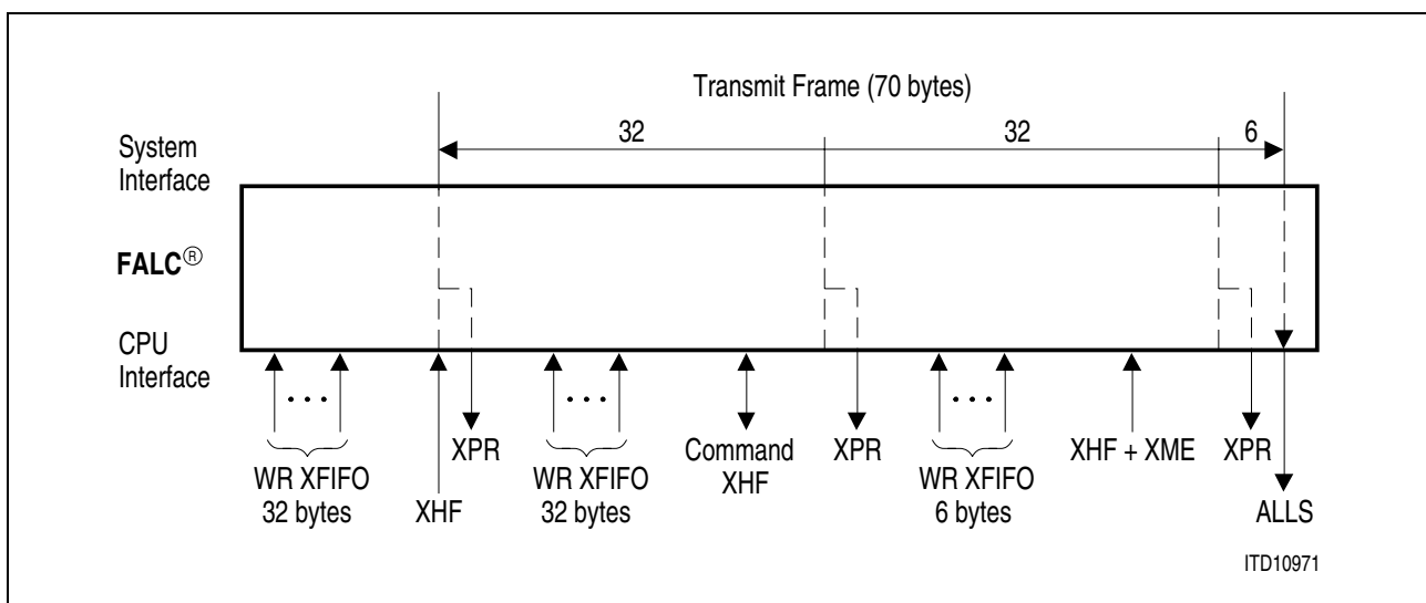
Figure 84 Interrupt Driven Transmission Example
