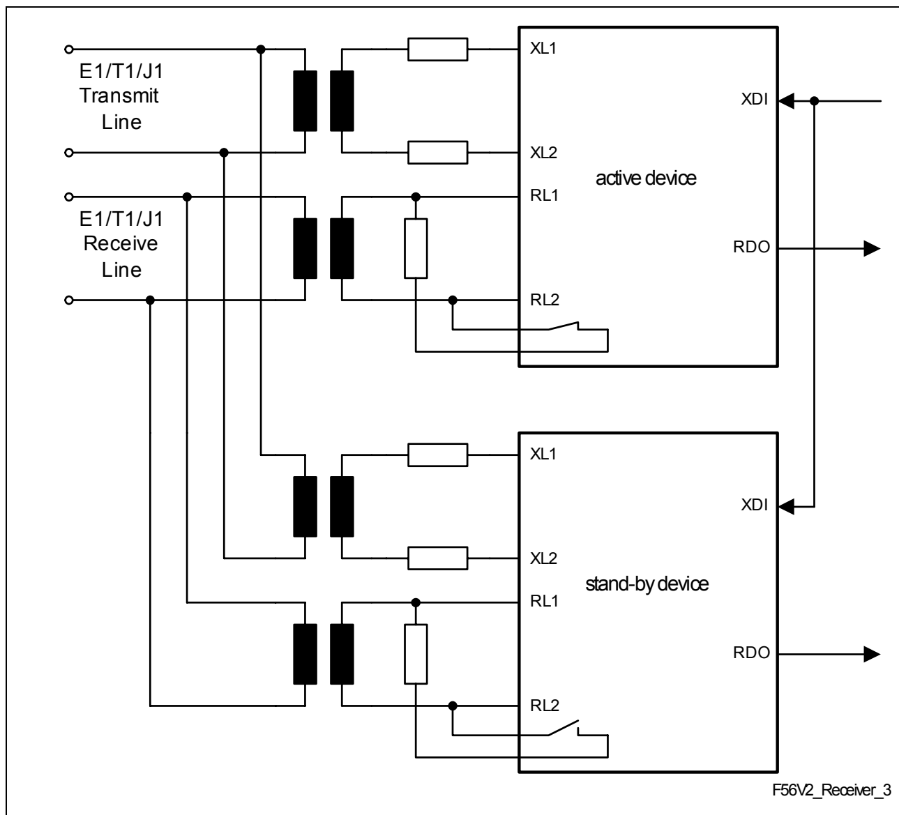
Figure 20 Long Haul Protection Switching Application (E1)
