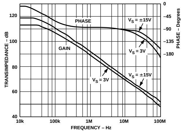
Figure 19. Open-Loop Transimpedance vs. Frequency (Relative to 1 Ω)
