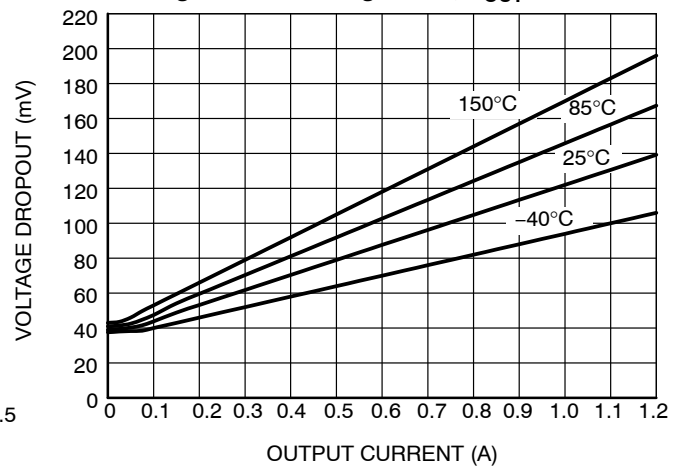
Figure 24. Dropout Voltage vs. Output Current, V_{OUT} = 3.3\text{ V}
