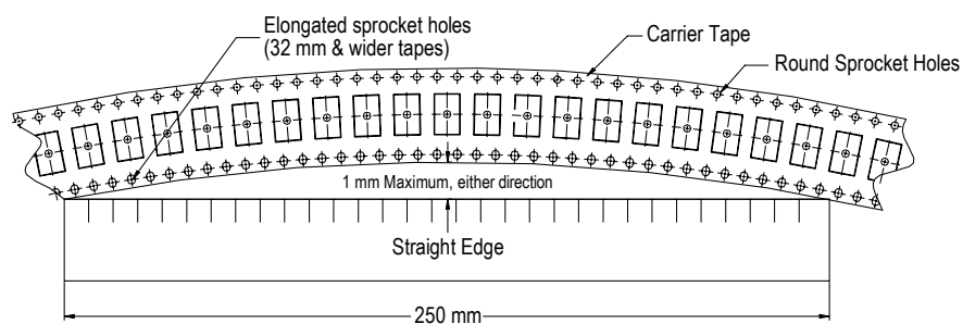
Figure 7 – Maximum Camber
