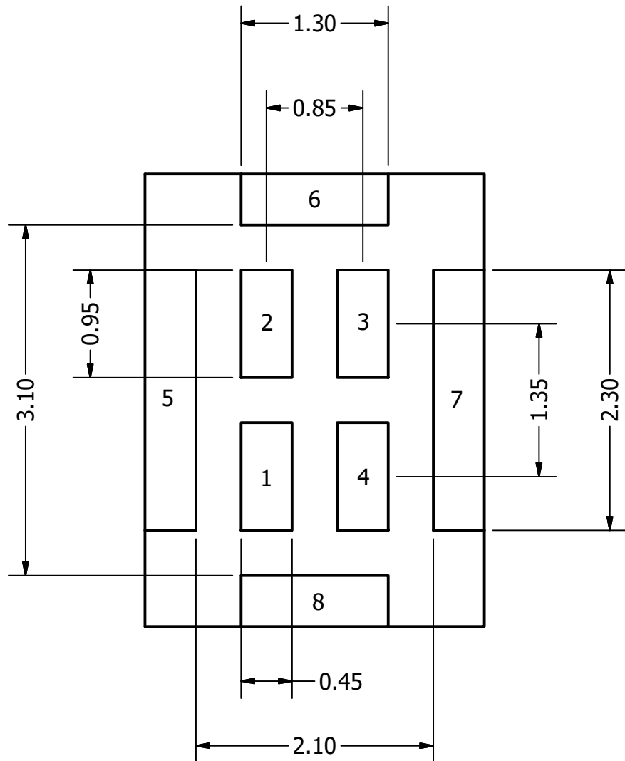
Bottom View
