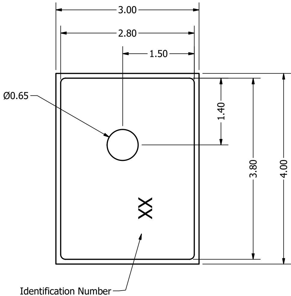
Top View
