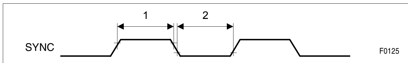
Figure 107 SYNC Timing
