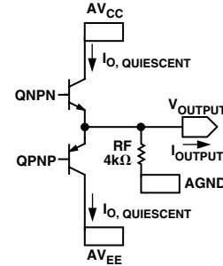
Figure 7. Simplified Output Stage
