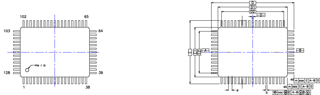
TOP VIEW
