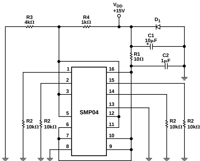
Figure 28. Burn-In Circuit
