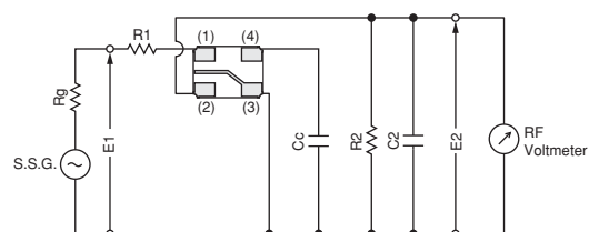
SFSKB2M80GF00-R1/SFSKB3M20FF00-R1
