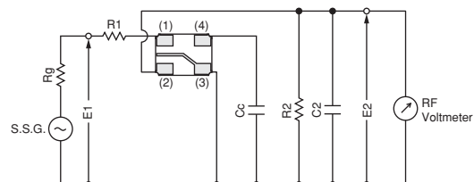
SFSKB4M80GF00-R1
