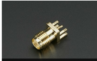
Edge-Launch SMA
