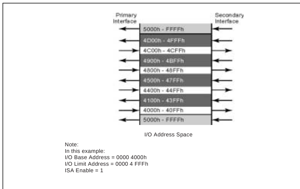
Figure 16. I/O Transaction Forwarding in ISA Mode
