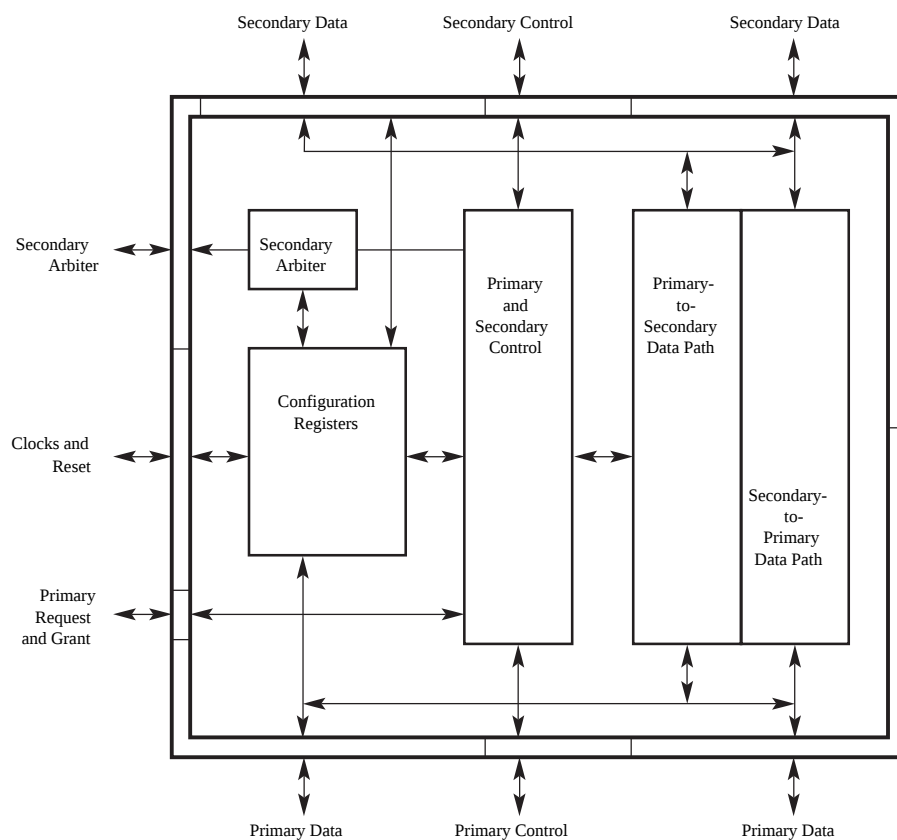
Figure 3. 21152 Block Diagram
