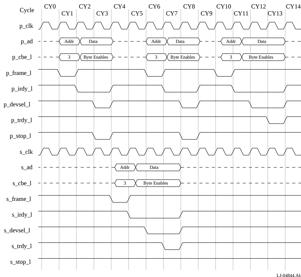
Figure 7. Downstream Delayed Write Transaction
