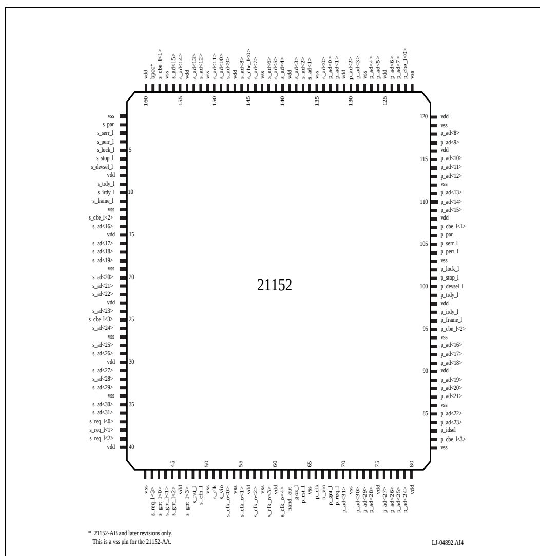
Figure 5. 21152 Pinout Diagram
