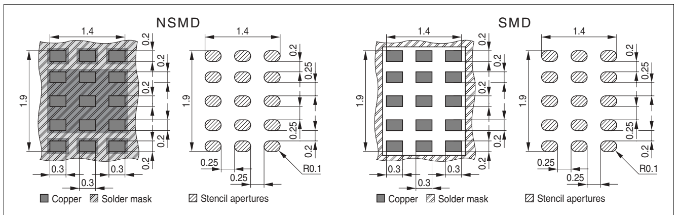
Figure 7 Recommended Land Pattern
