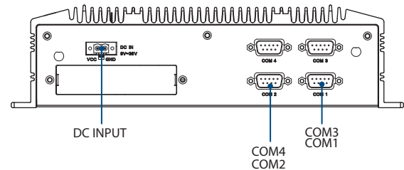
Rear Panel External I/O Mechanical Layout/Drawing
