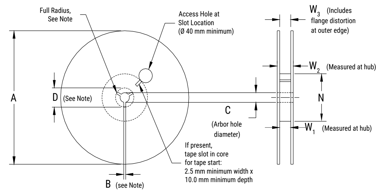
Figure 5 – Reel Dimensions
