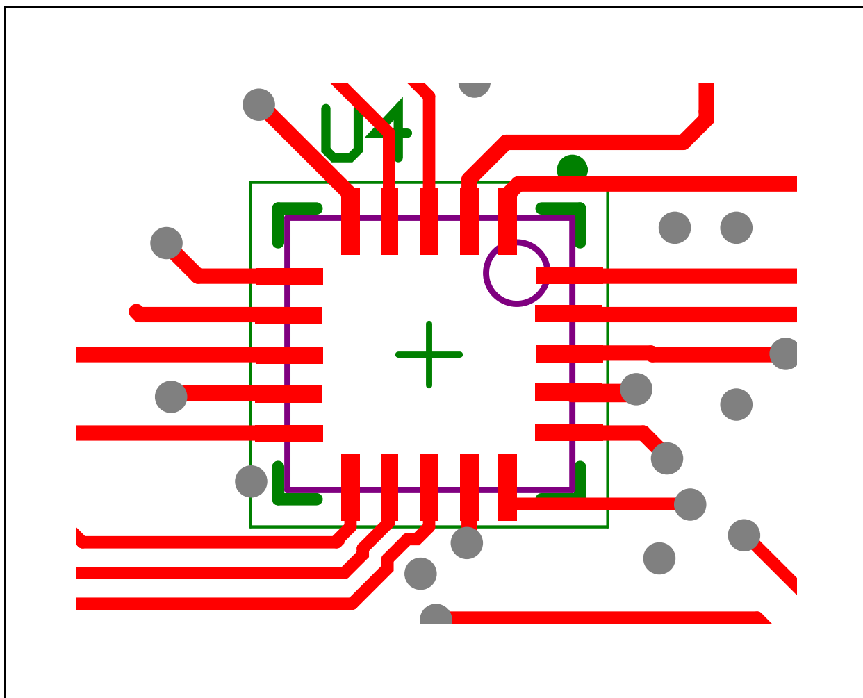
Figure 22: Typical Layout Routing
