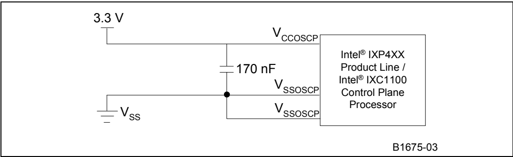
Figure 10. V_{CCOSC} Power Filtering Diagram
