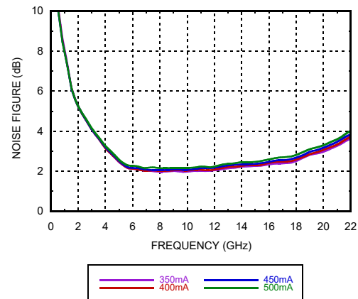
Noise Figure vs. Idd
