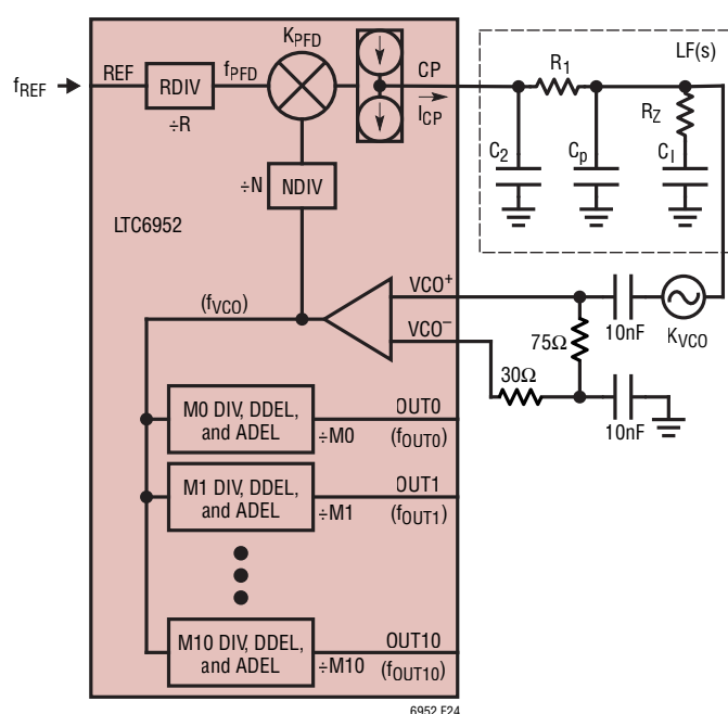
Figure 24. PLL Loop Diagram
