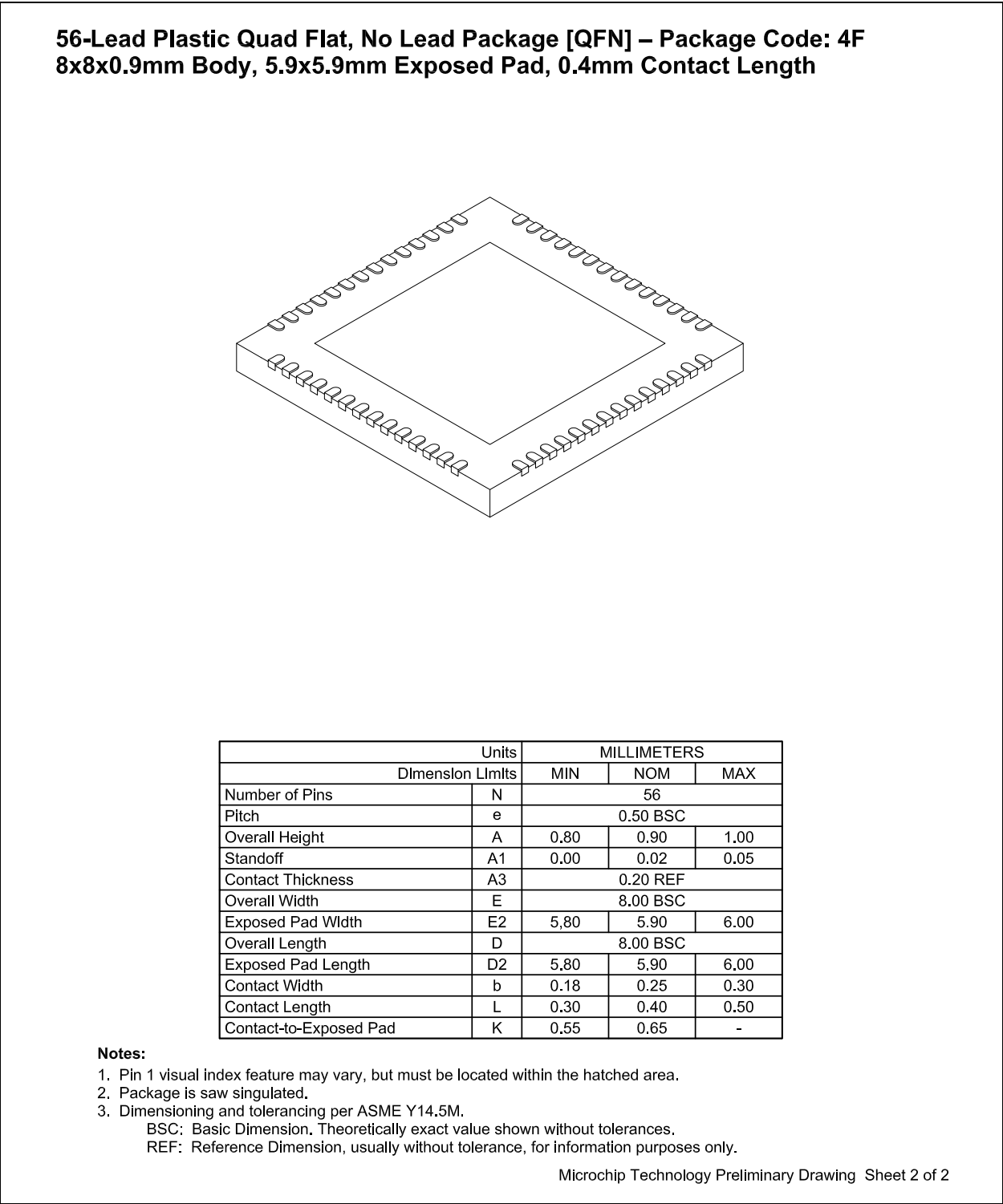
FIGURE 17-2: 56-SQFN PACKAGE (DIMENSIONS)
