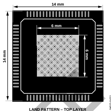
Figure 21. Land Pattern—Top Layer
