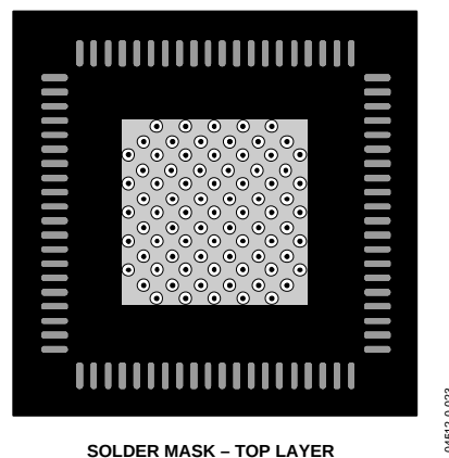
Figure 23. Solder Mask—Top Layer
