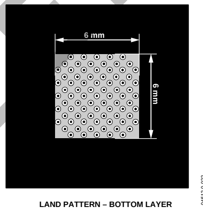
Figure 22. Land Pattern—Bottom Layer
