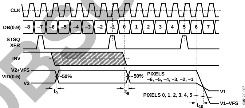
Figure 7. Output Timing (R/L = Low, E/O = High)
